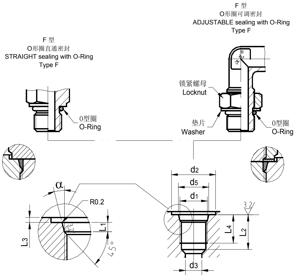
SAE J1926-1 Port Detail (ISO 11926-1)
